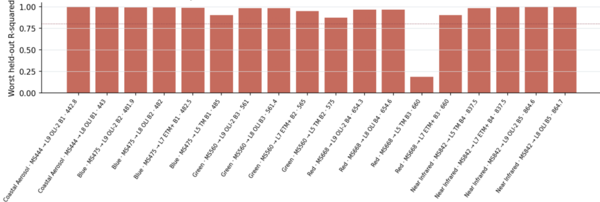
Leave-one-site-out transferability
