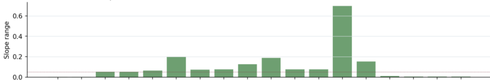
Leave-one-site-out transferability
